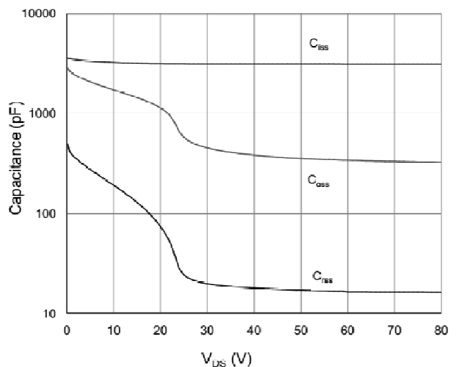
Capacitance
