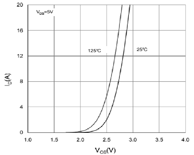
Transfer Characteristic
