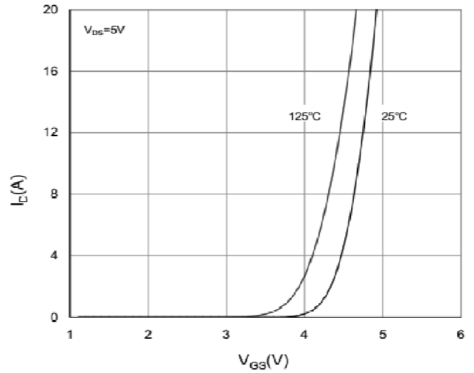
Transfer Characteristic
