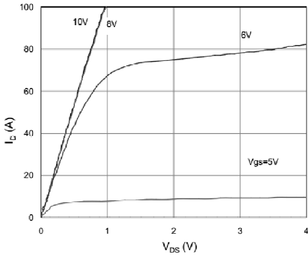
Output Characteristic
